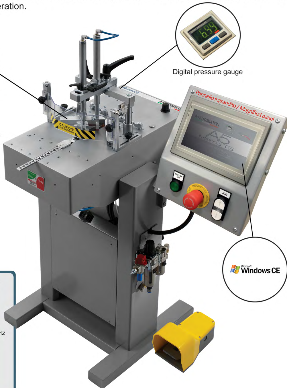
Adjustable tilting fence with special "frame tightening" device
